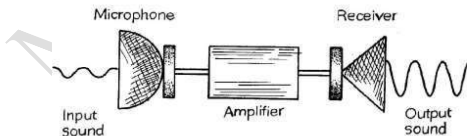
Figure 3.3: (i) Basic structure of Hearing Aid.
