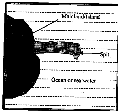
Figure 28: A Spit
