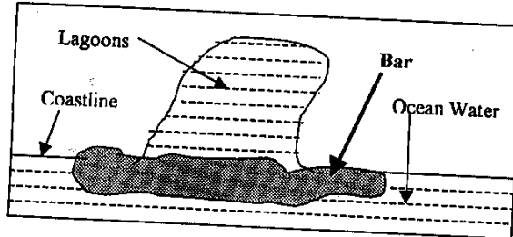
Figure 29: A Bar
