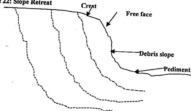
Figure 22: Slope Retreat
