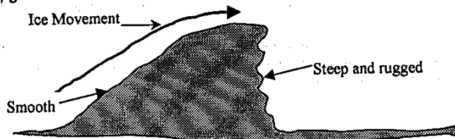
Figure 18: Rock Moutonnee
