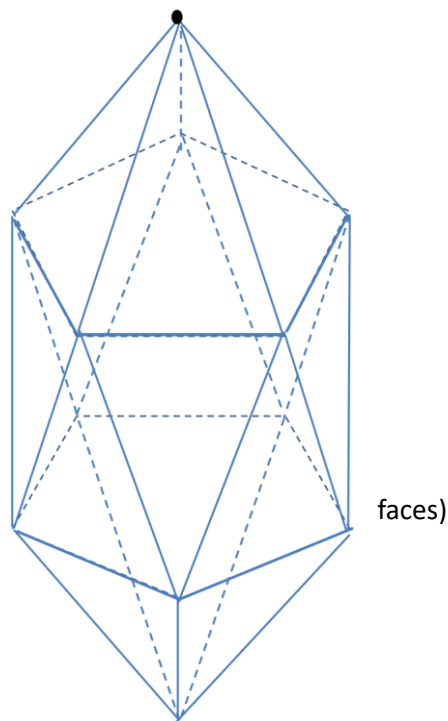
Icosahedron (20
