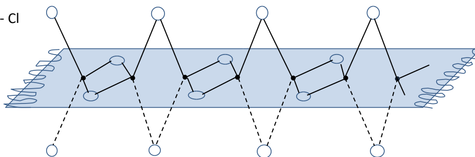
Polymer (\text{BeCl}_2)_n
