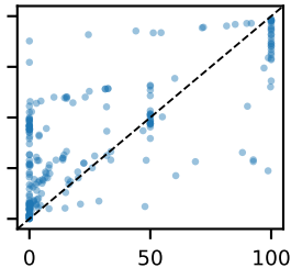
locked test
