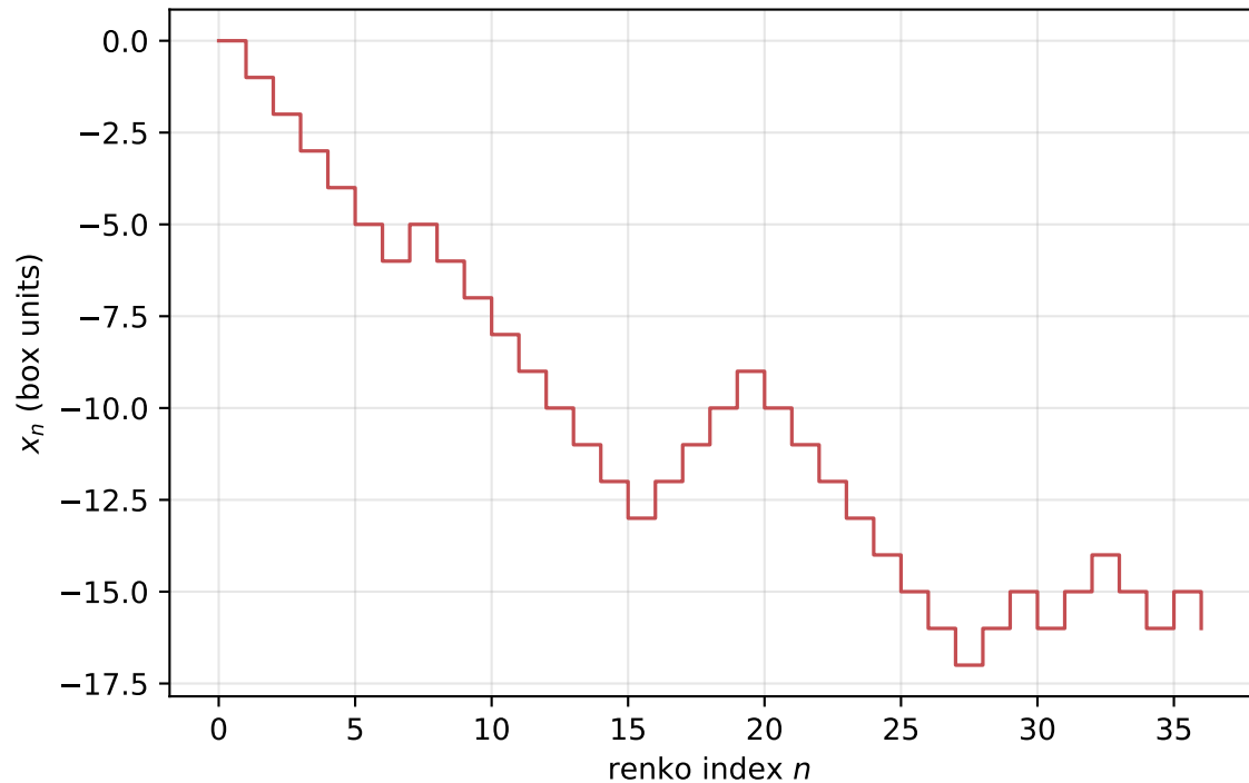
average renko ( B = 2 )
