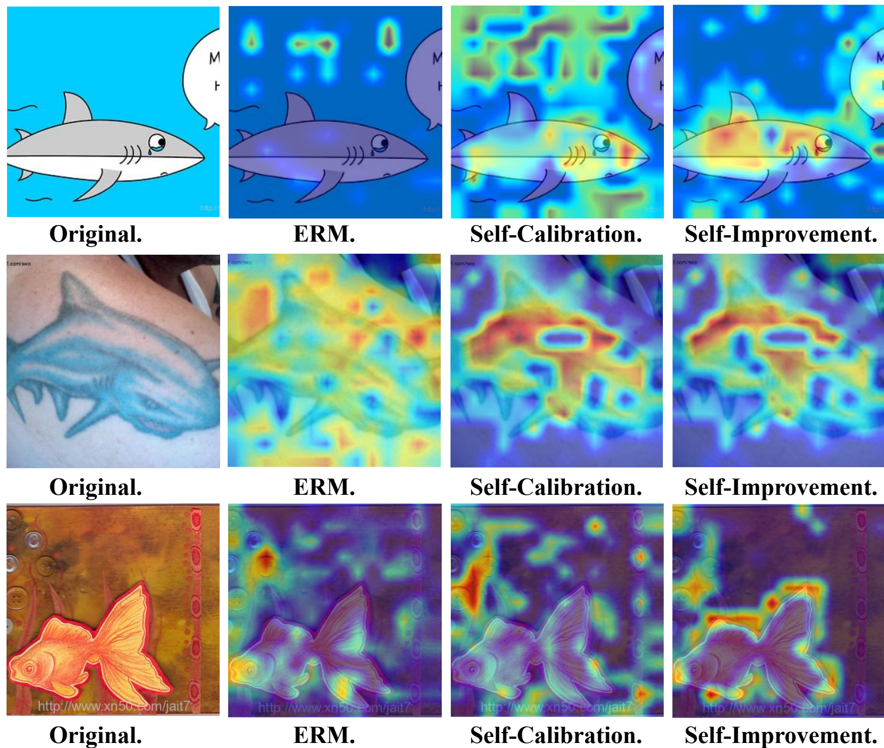
Figure: The saliency maps in IN-R+W. From left to right in each case are from the original image, the pre-trained ViT-Large, the source model with self-calibration strategy, and the target model with self-improvement strategy. warm colors indicate a high level of attention for models. It can be seen that calibration loss enriches feature distribution, resulting in the source model focusing on more locations. The self-improvement strategy further forces the model to focus on true underlying features by random mask strategy and adaptive attention alignment module.
