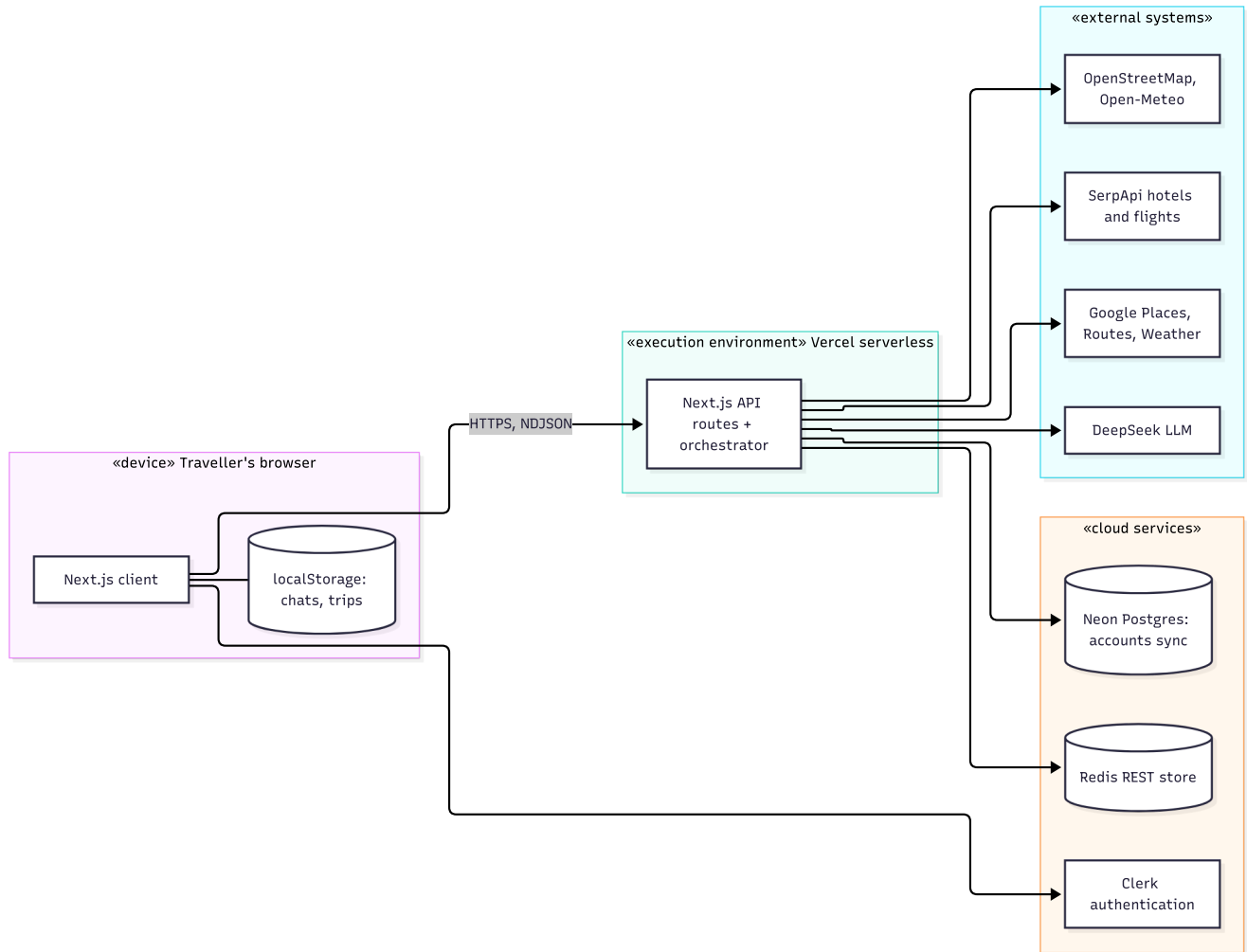
Figure 5.4. Deployment diagram.
