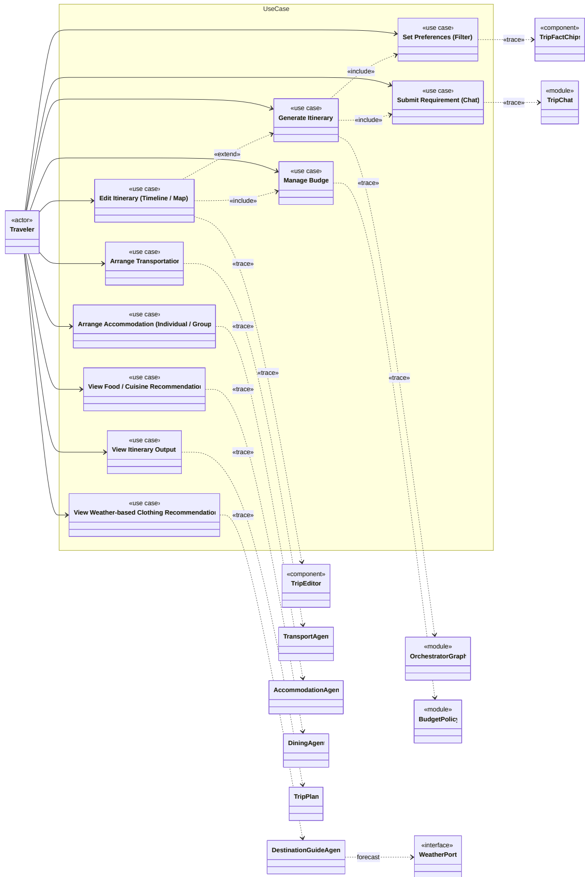
Figure 6.5. Diagram 5: use cases traced onto the model.
