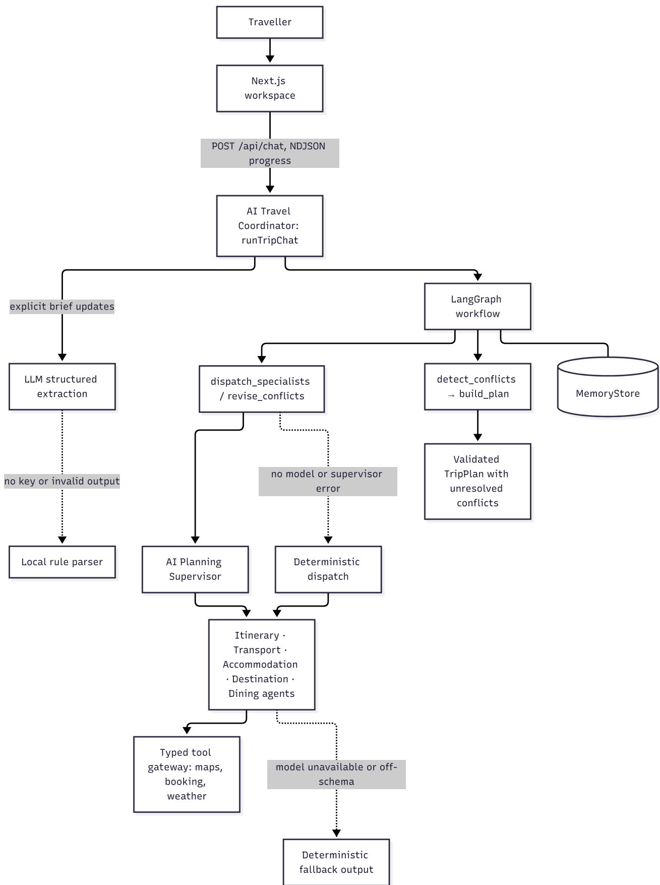
Figure 5.1. Runtime flow.
