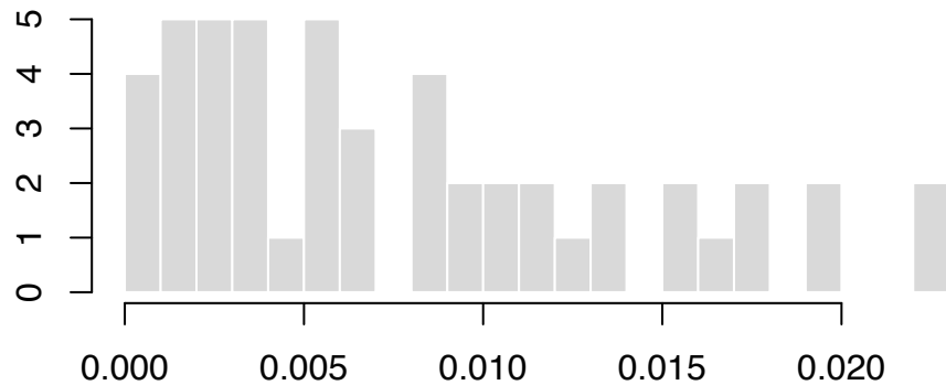
Permutation (p=0)
