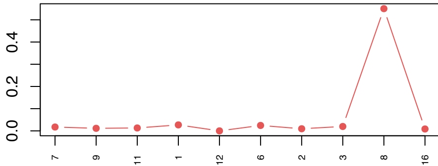
CTS 8 (51 genes)
