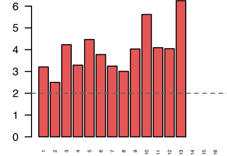
Cluster 3 16 modules
