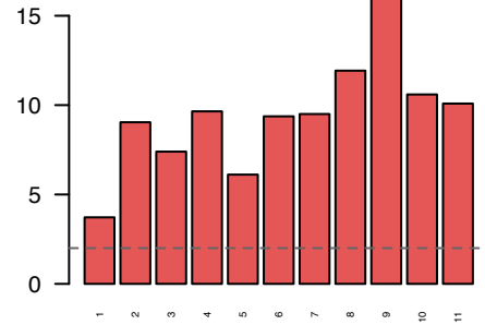
Cluster 6 11 modules
