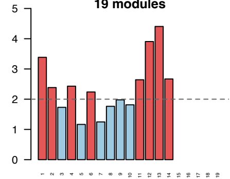
Cluster 2 19 modules
