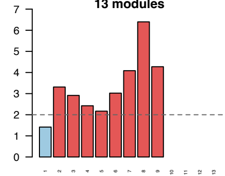
Cluster 8 13 modules
