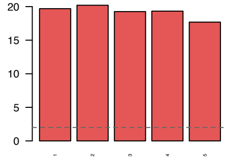
Cluster 16 5 modules
