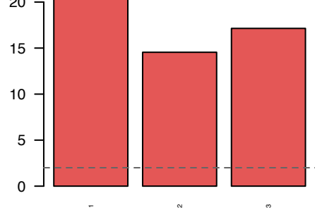
Cluster 3 16 modules
