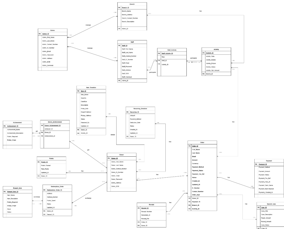
Figure 161: Entity Relationship Diagram
