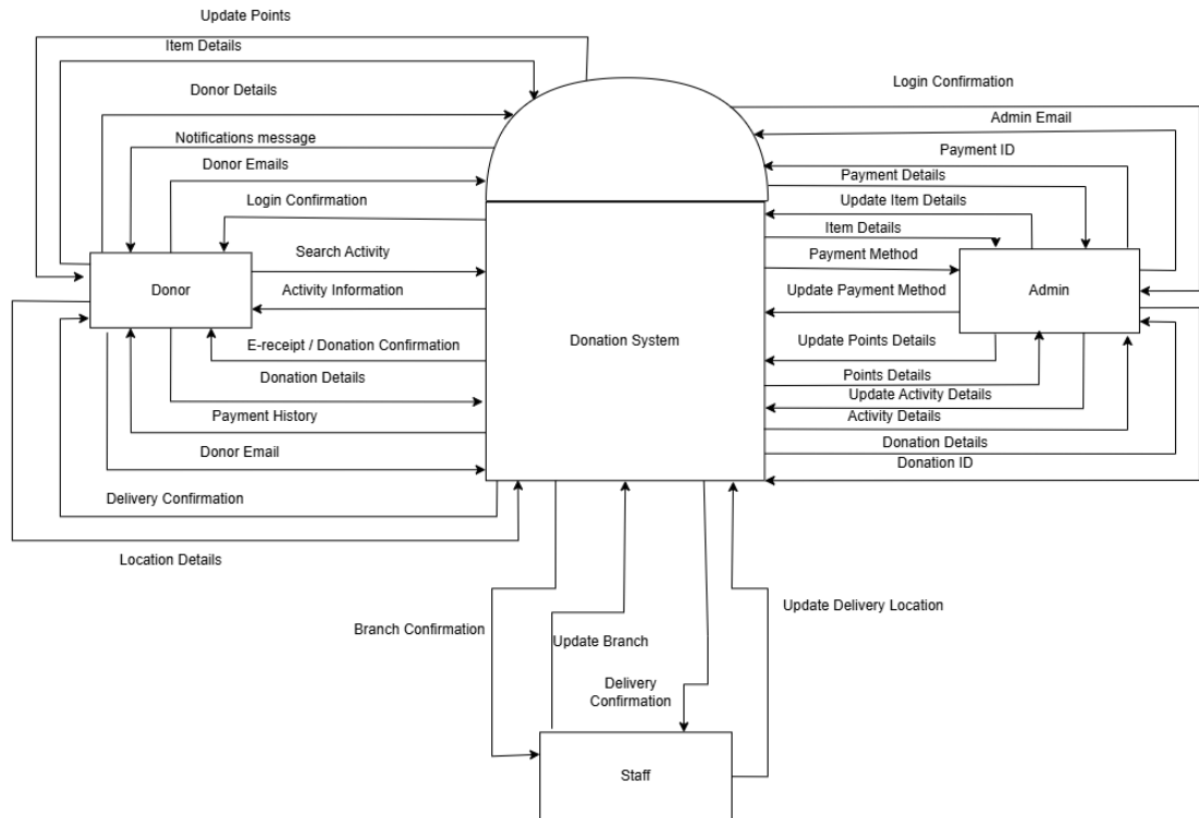
Figure 159: Context Diagram for Donation System
