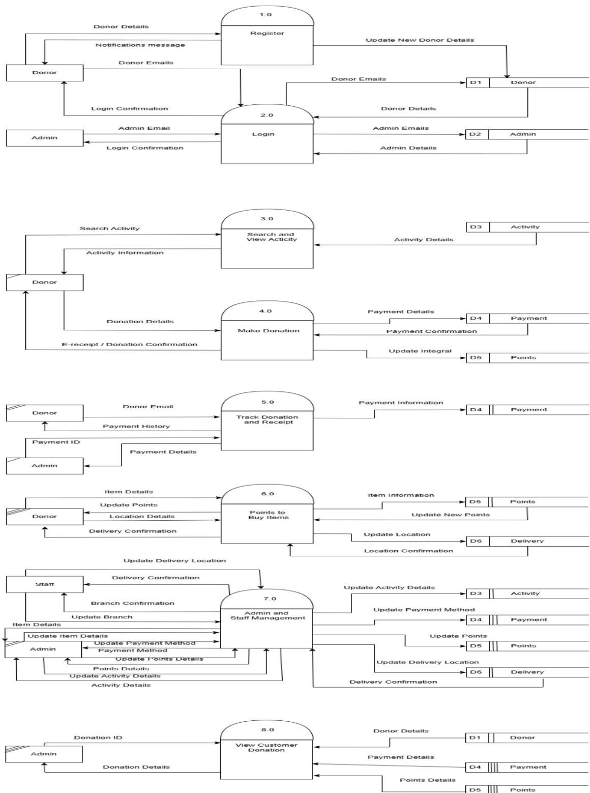
EFigure 160: Data Flow Diagram for Donation System
