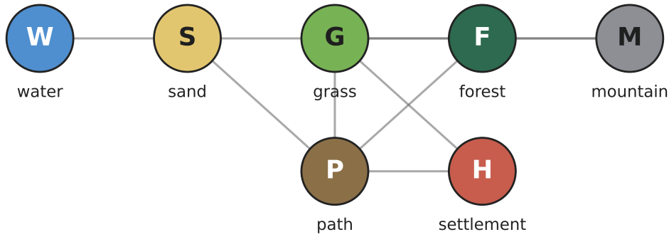
Figure 2.1.3: All different node types and how they are constrained. Each edge represents which node types can be adjacent in the domain.
