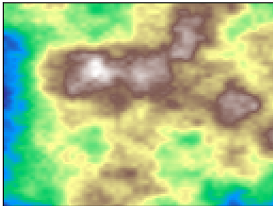
balanced
