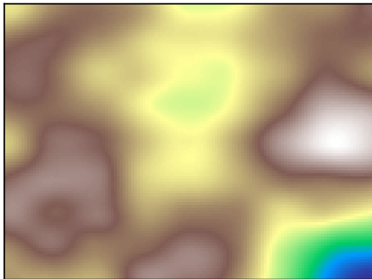
smooth
