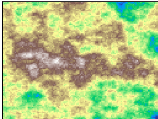
rugged
