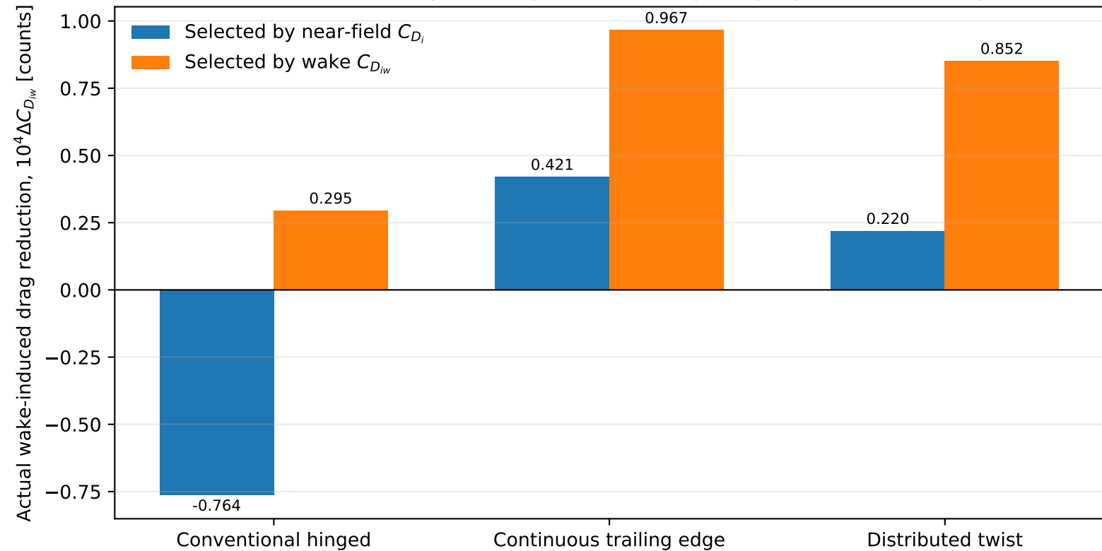
Corrected Mach-0.1 study: consequence of using the proper induced-drag metric
