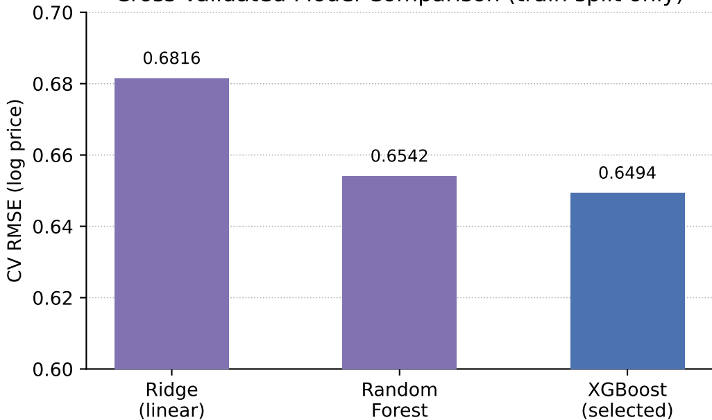
Cross-Validated Model Comparison (train split only)
