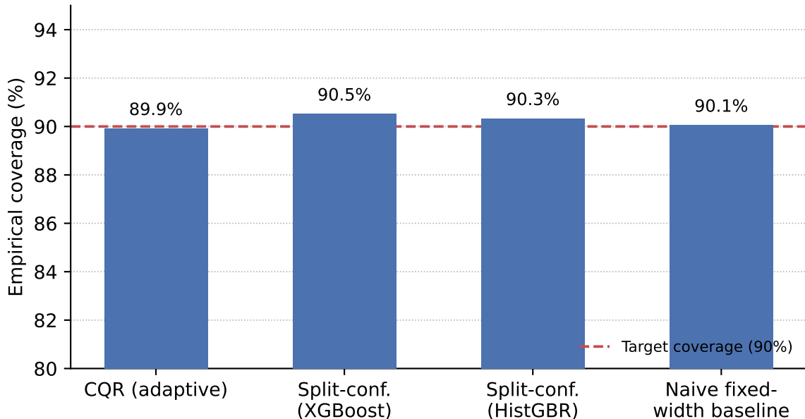
90% Interval Coverage by Method (India, test set)
