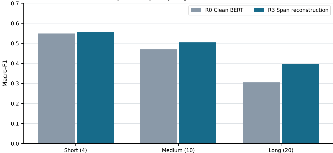
All three modalities: middle-position span by length
