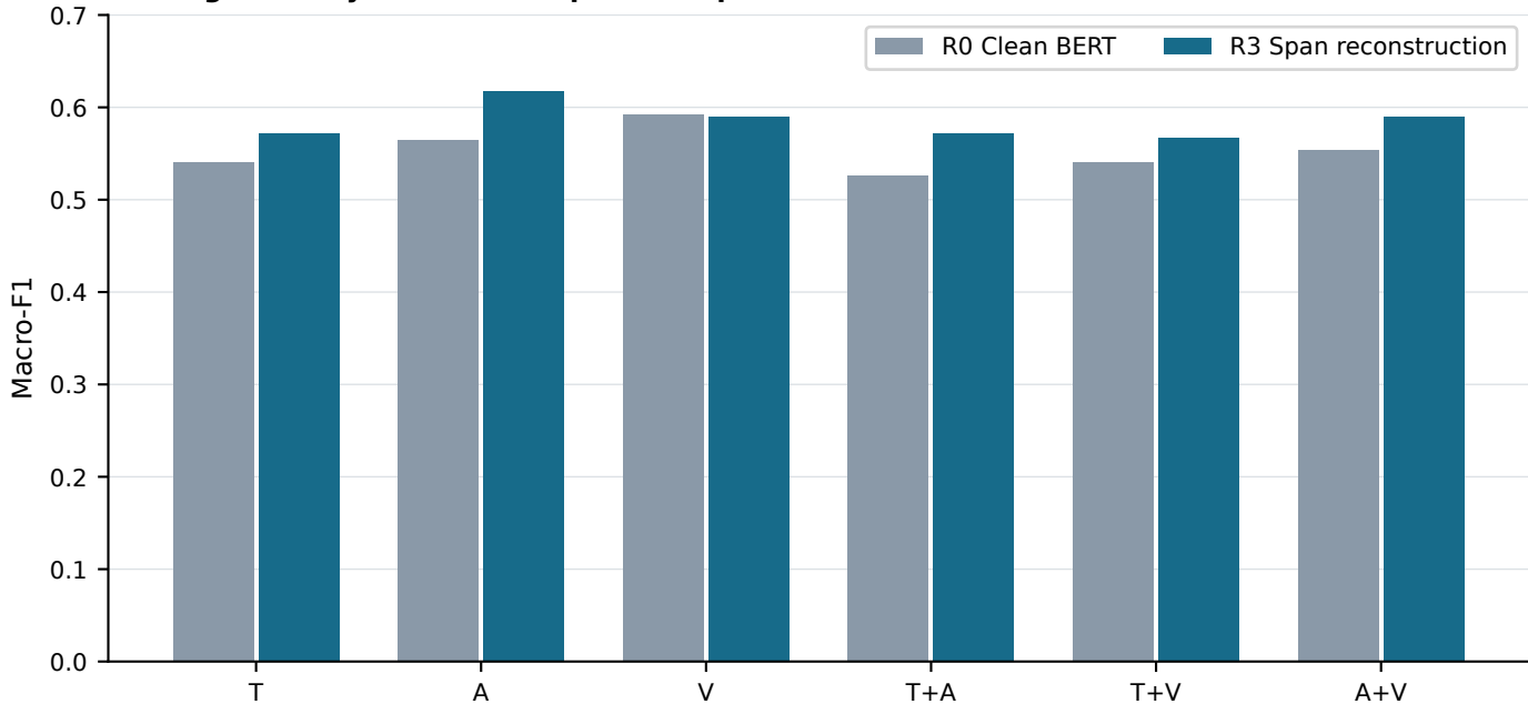
Missing modality: 30% middle-position span
