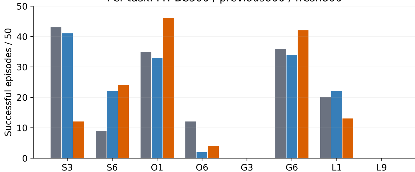
Per-task: MT-BC300 / previous600 / fresh800
