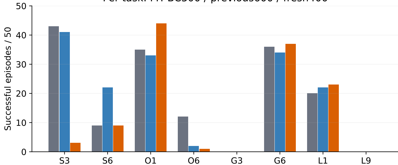
Per-task: MT-BC300 / previous600 / fresh400
