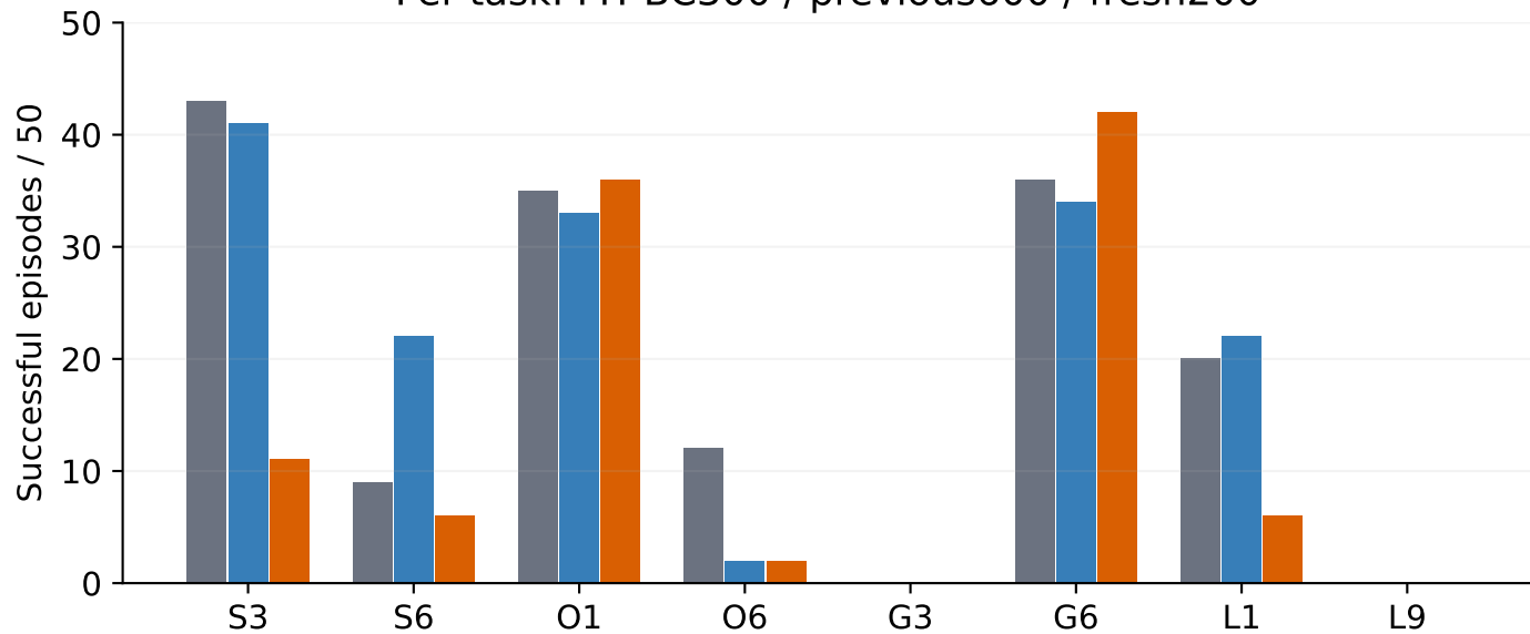
Per-task: MT-BC300 / previous600 / fresh200
