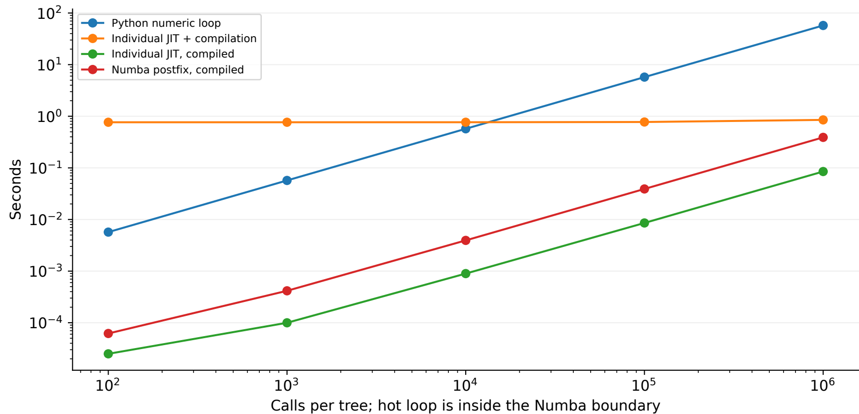
Individual JIT: compilation amortization (sum over 8 trees)
