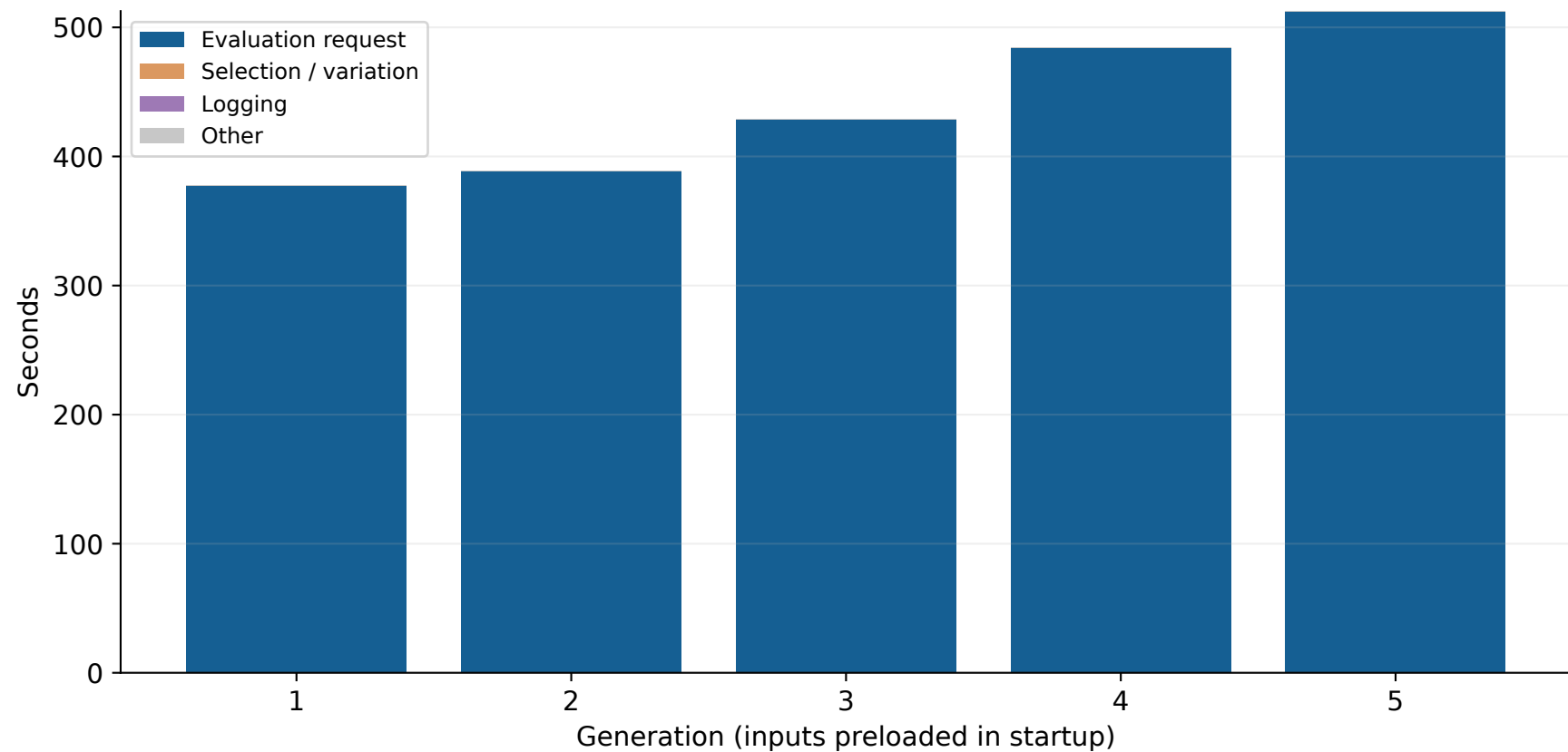
Real evolution: CPU-8 (FP64) (repeat 0)
