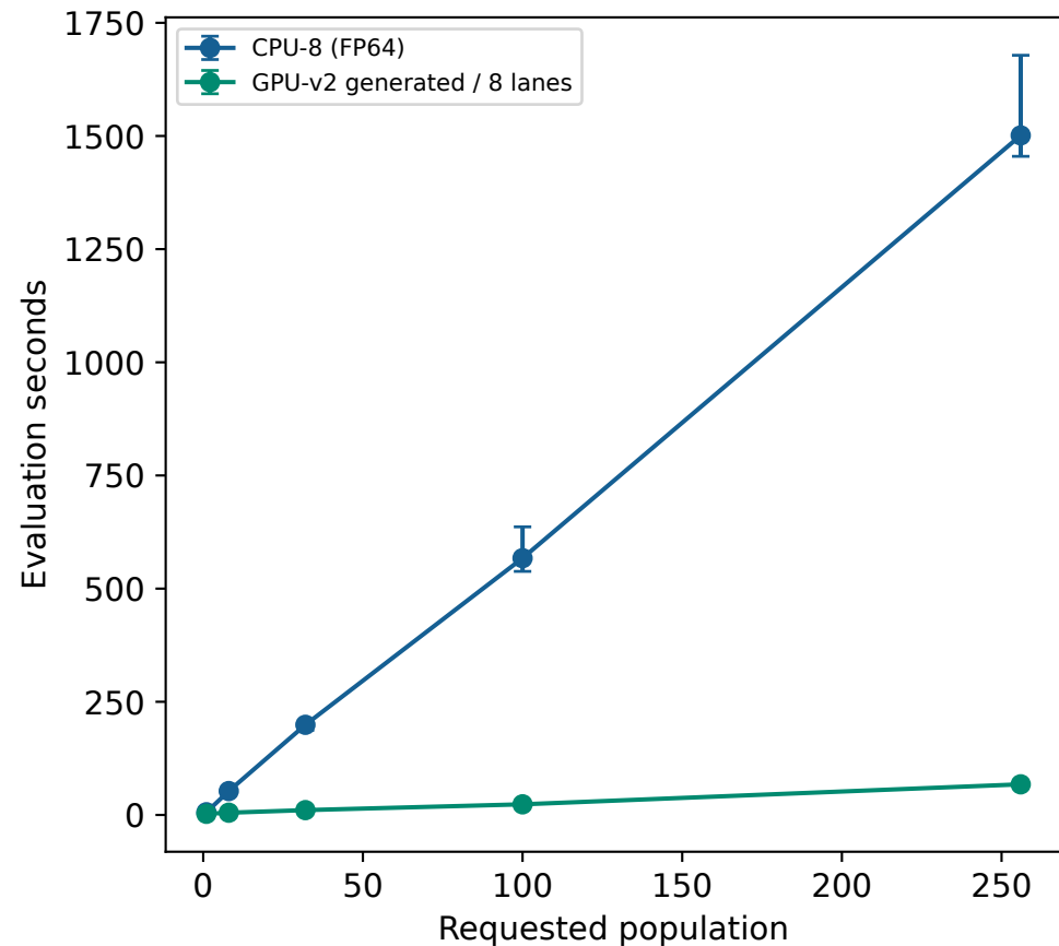
Population scaling (TSP100, 32 instances)
