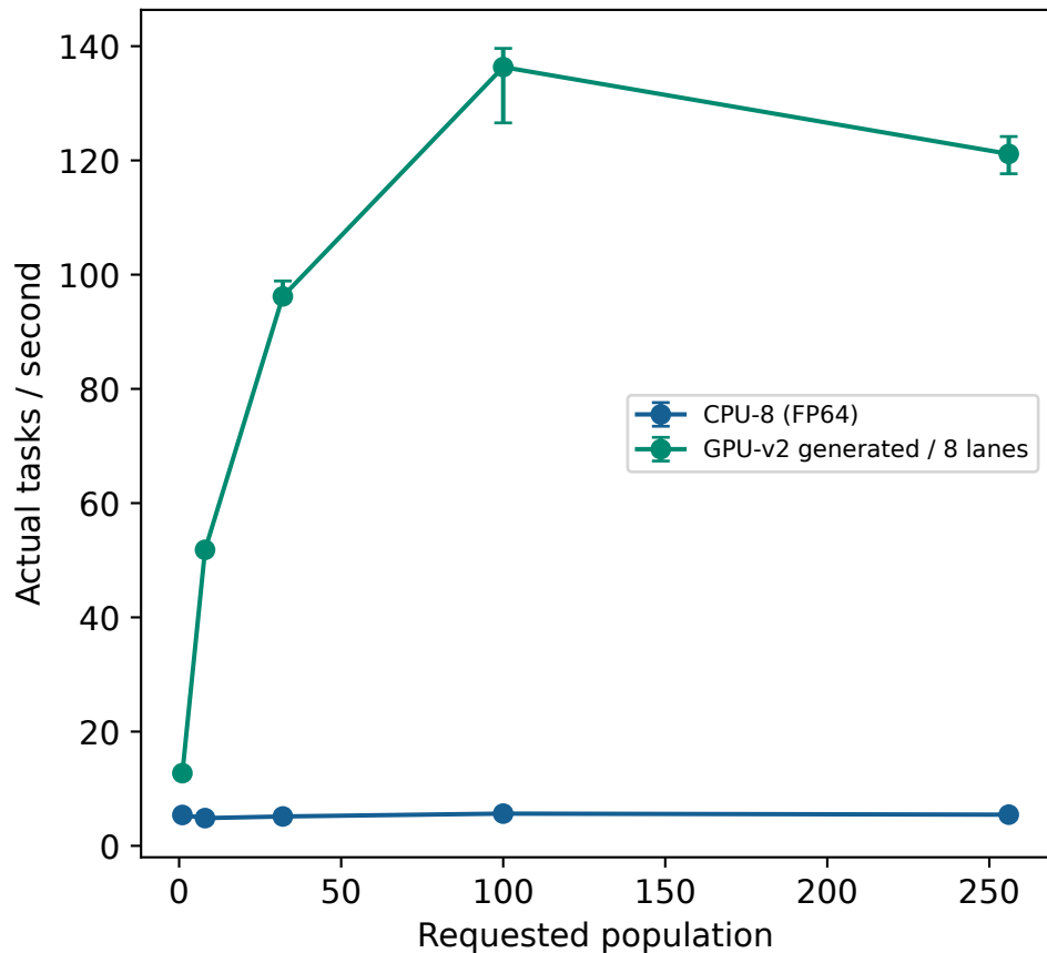
Population scaling (TSP100, 32 instances)
