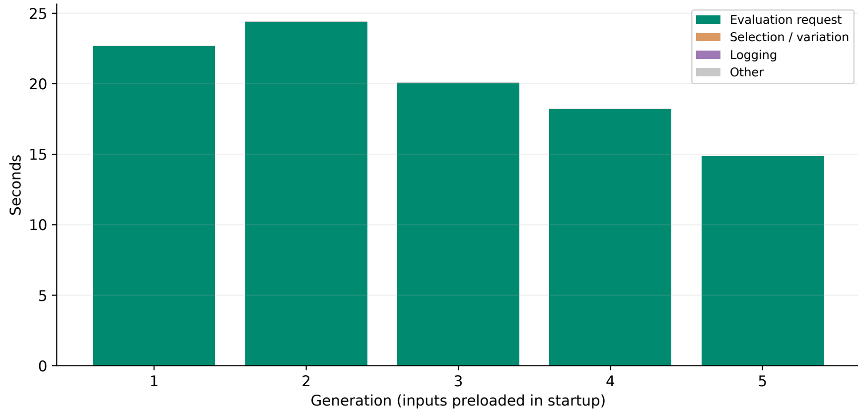
Real evolution: GPU-v2 generated / 8 lanes (repeat 2)
