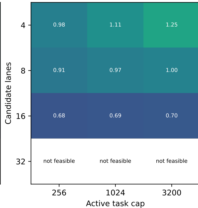
TSP100 / cohort g25
