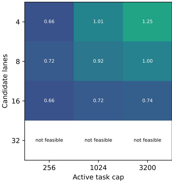
TSP100 / cohort g1
