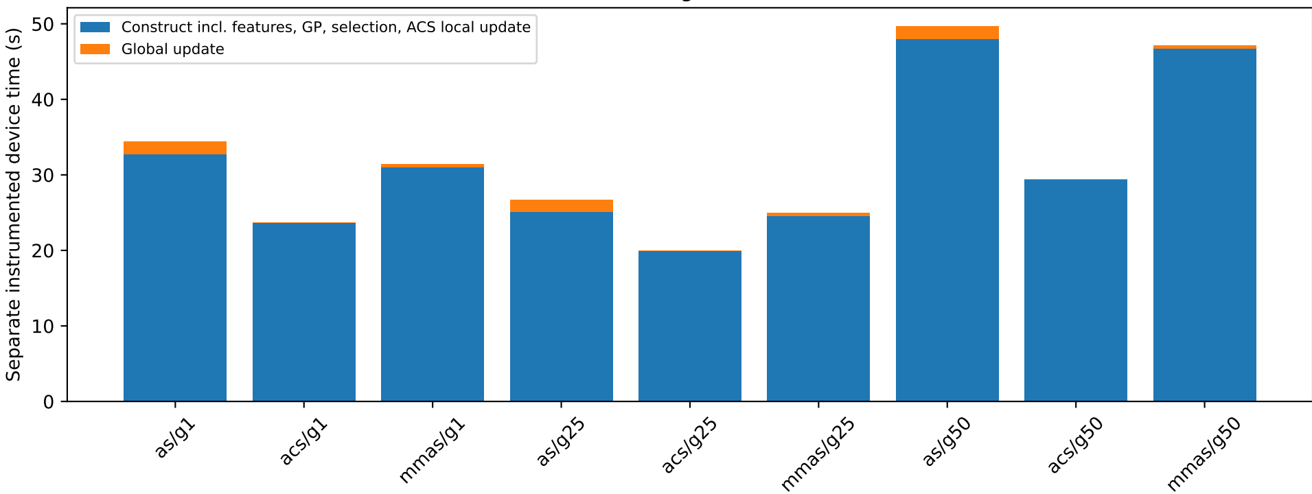
TSP100: stage attribution
