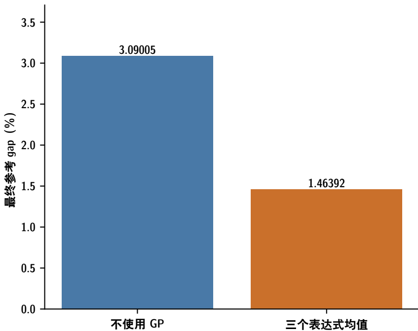
AS + 2-opt
