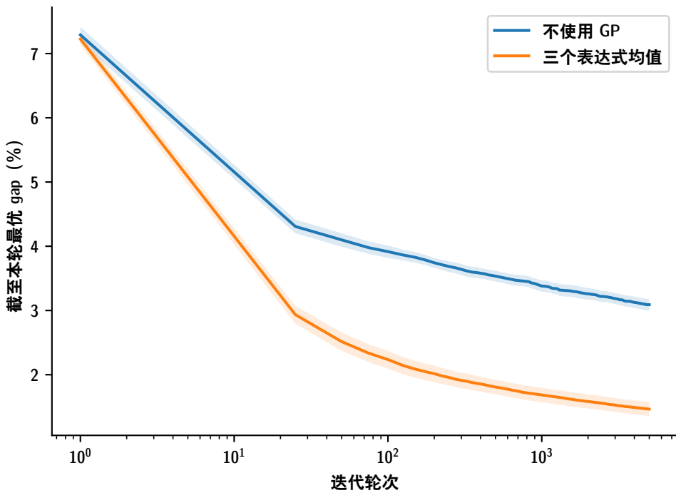
AS + 2-opt
