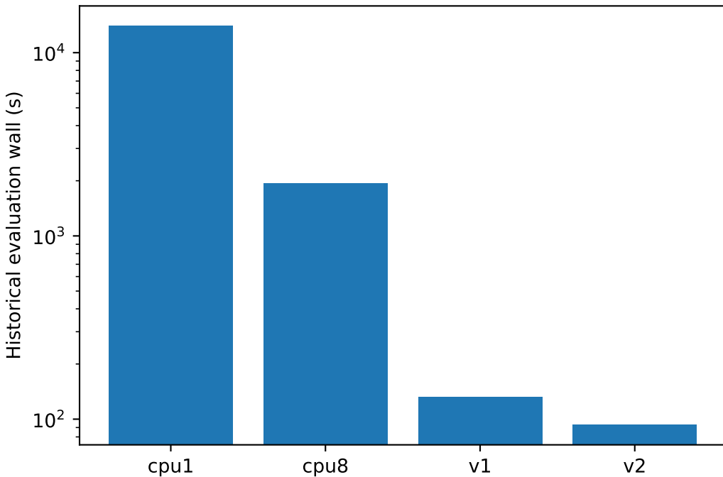
TSP100 / 5-generation trace
