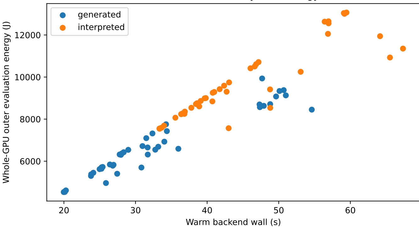
TSP100; not whole-system energy
