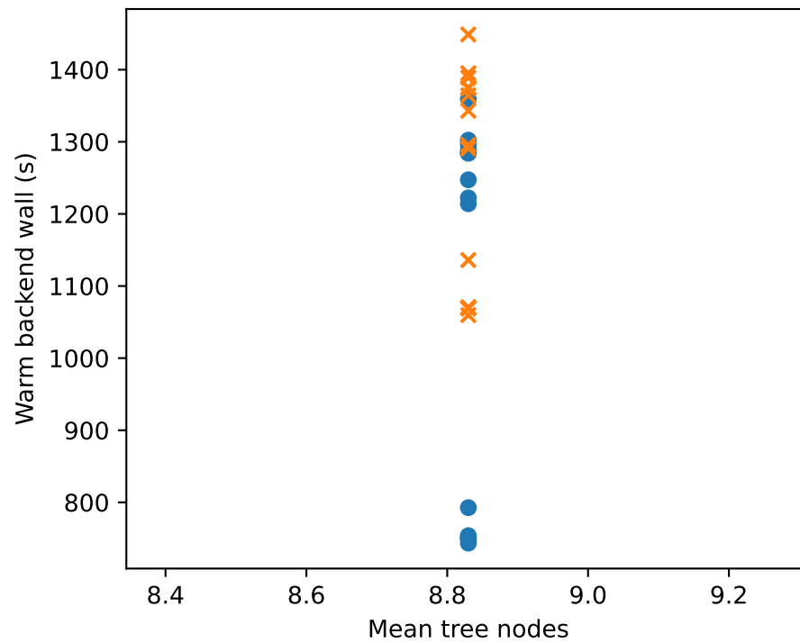
TSP500: descriptive associations, not causal attribution
