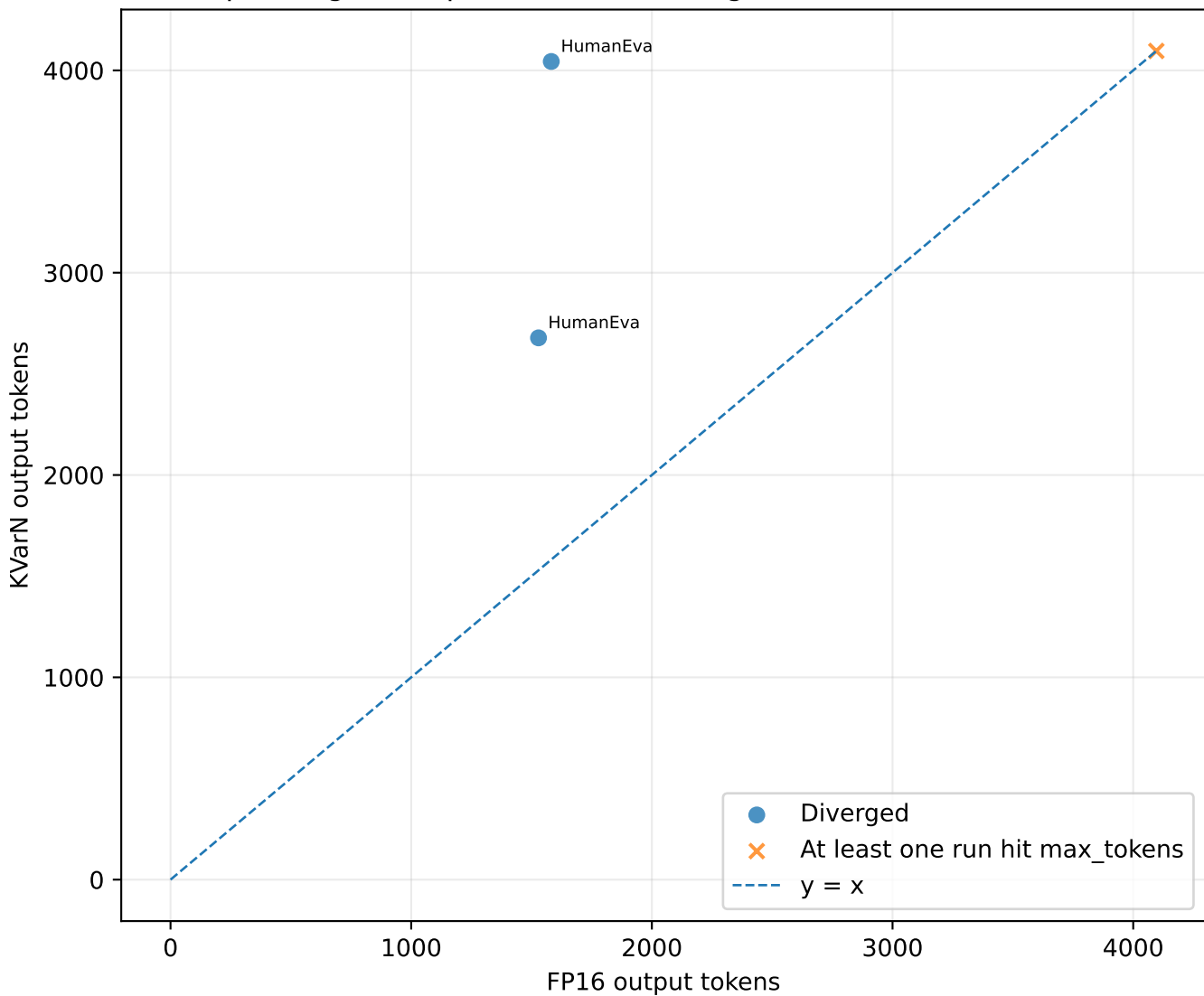
Output length comparison (n=3, divergence=100.0%, censored=1)
