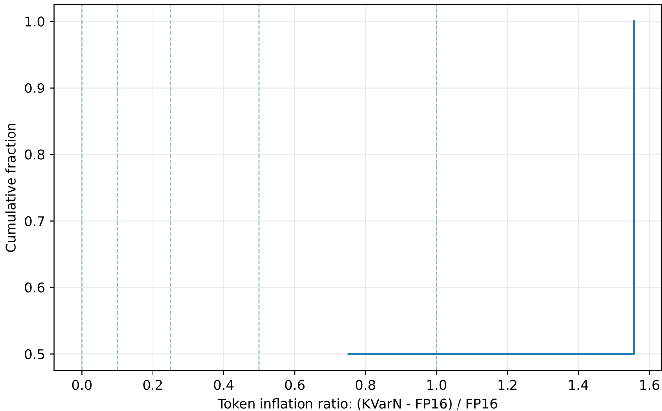
HumanEval token-inflation CDF
