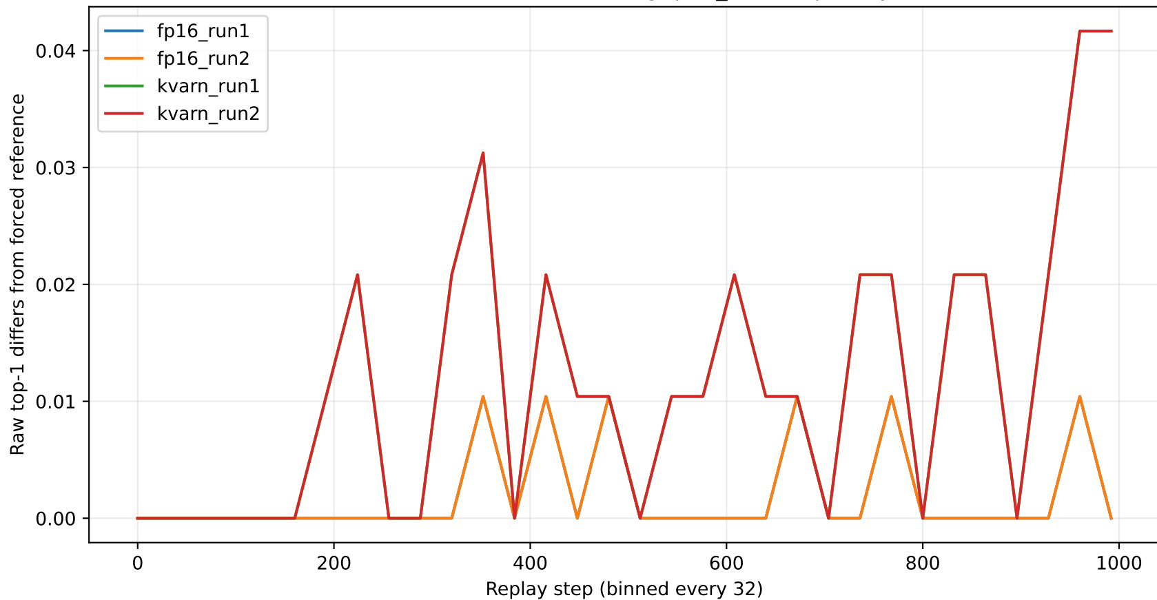
Reference adherence along fp16_run1 trajectory
