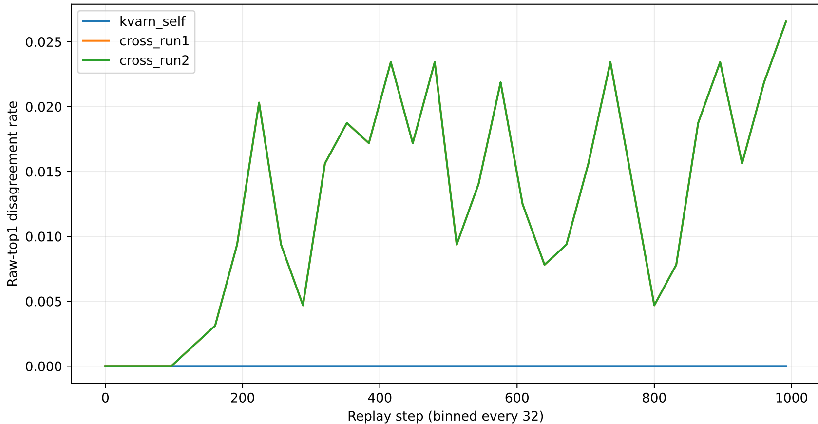
Aligned replay disagreement rate over generation
