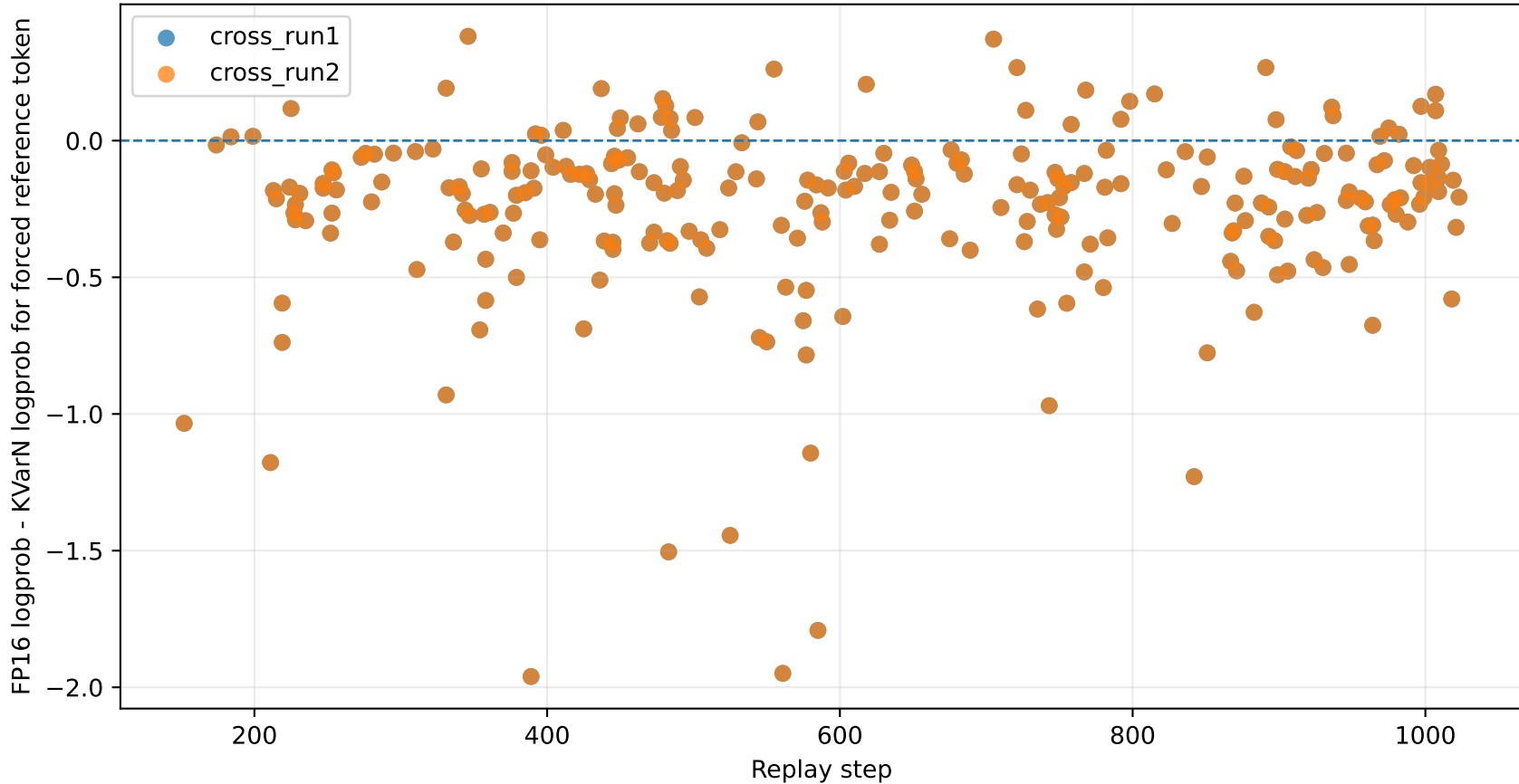
Reference-token probability shift at cross-mode top-1 flips
