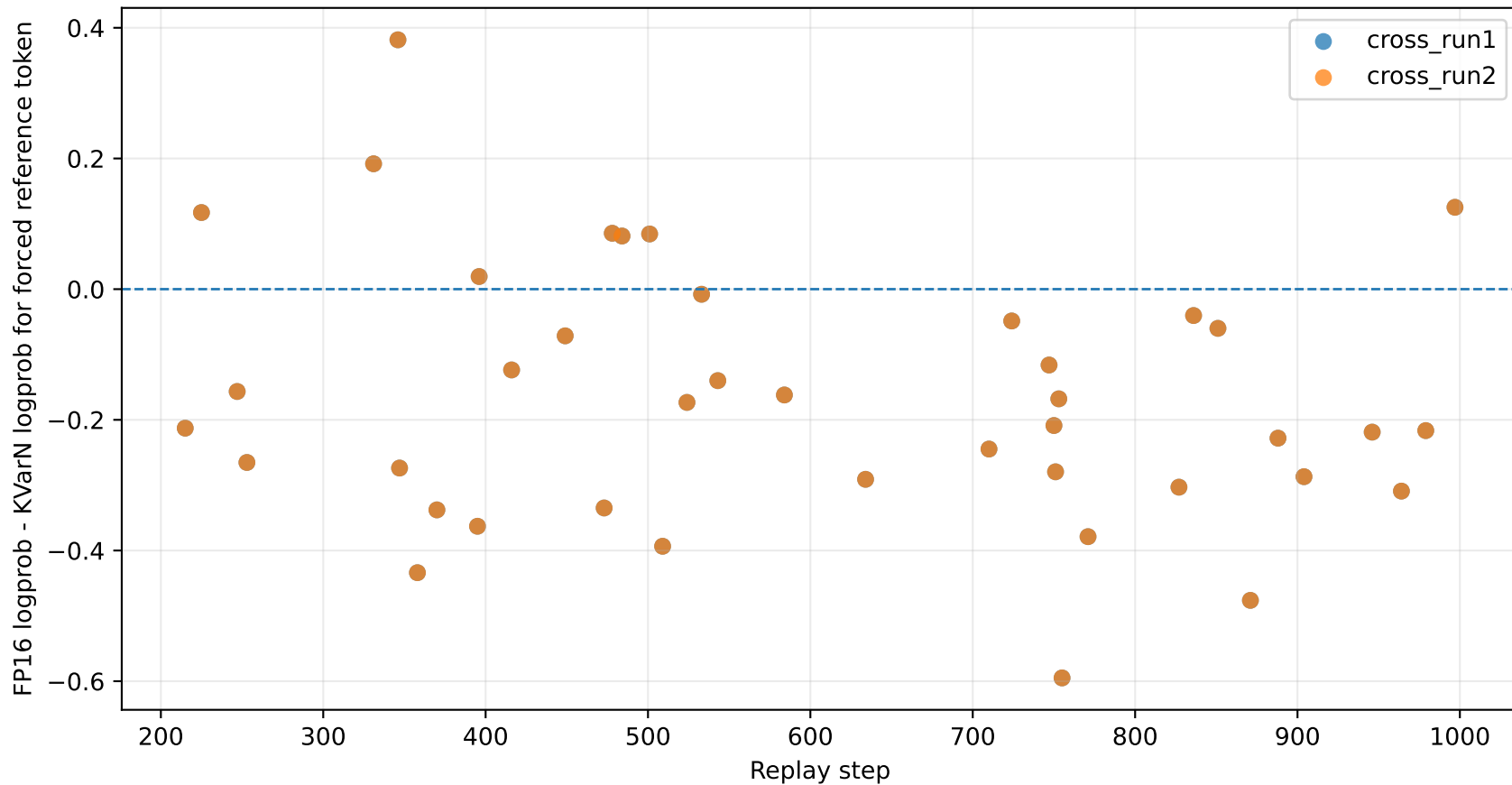
Reference-token probability shift at cross-mode top-1 flips
