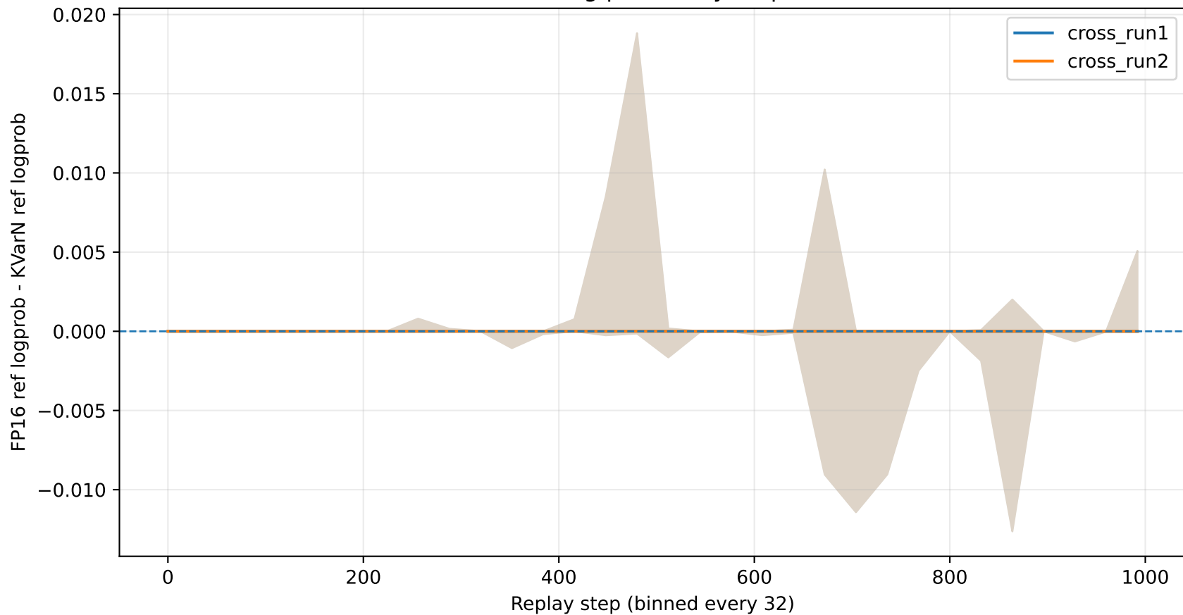
Reference-token log-probability drop under KVarN
