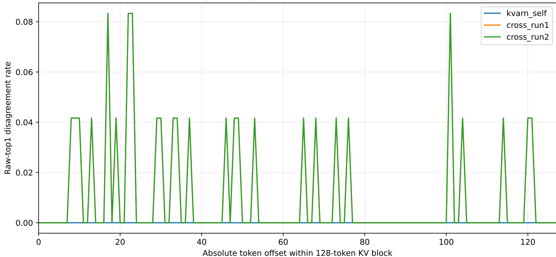
Aligned disagreement versus KV-block offset
