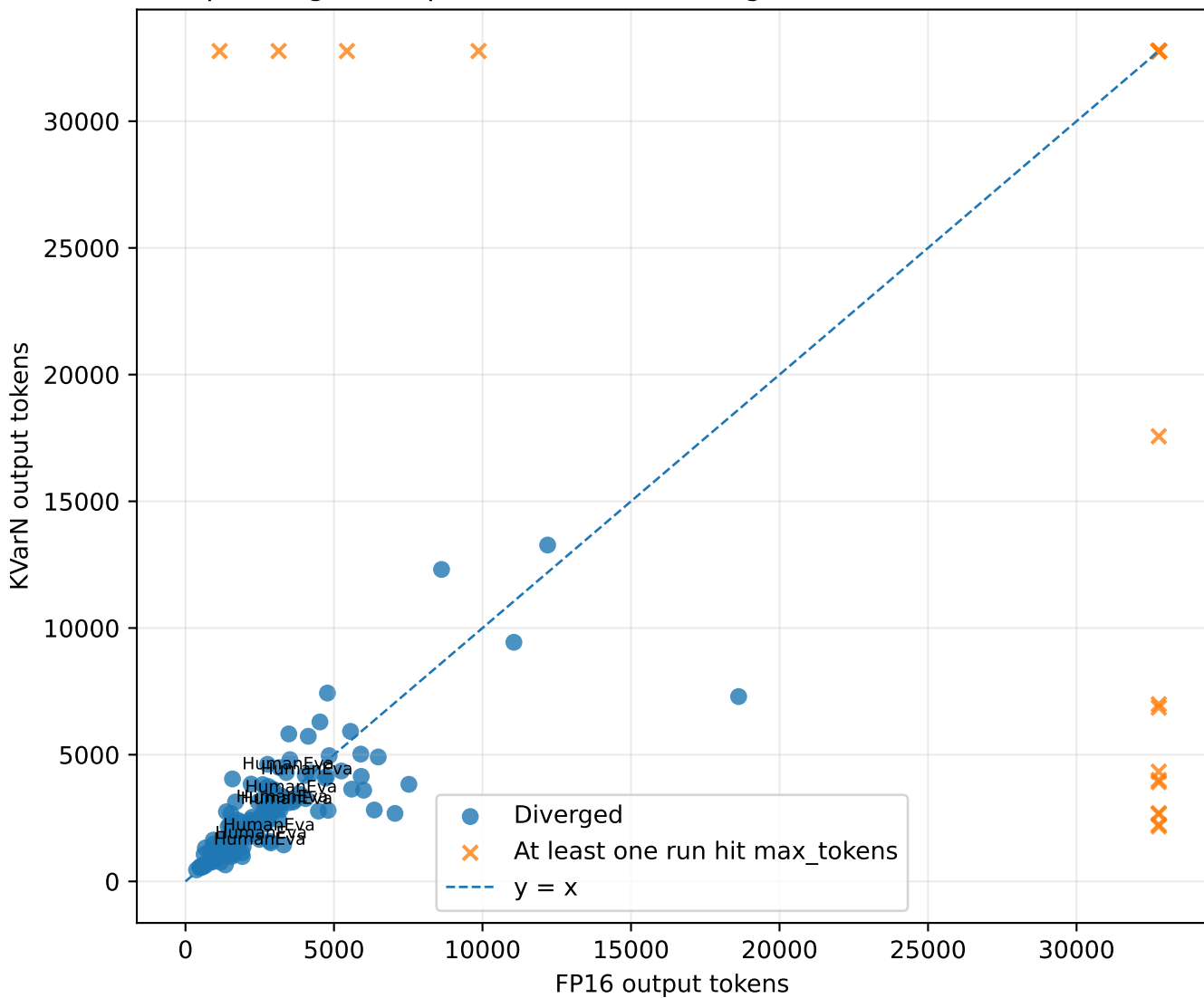
Output length comparison (n=164, divergence=100.0%, censored=26)
