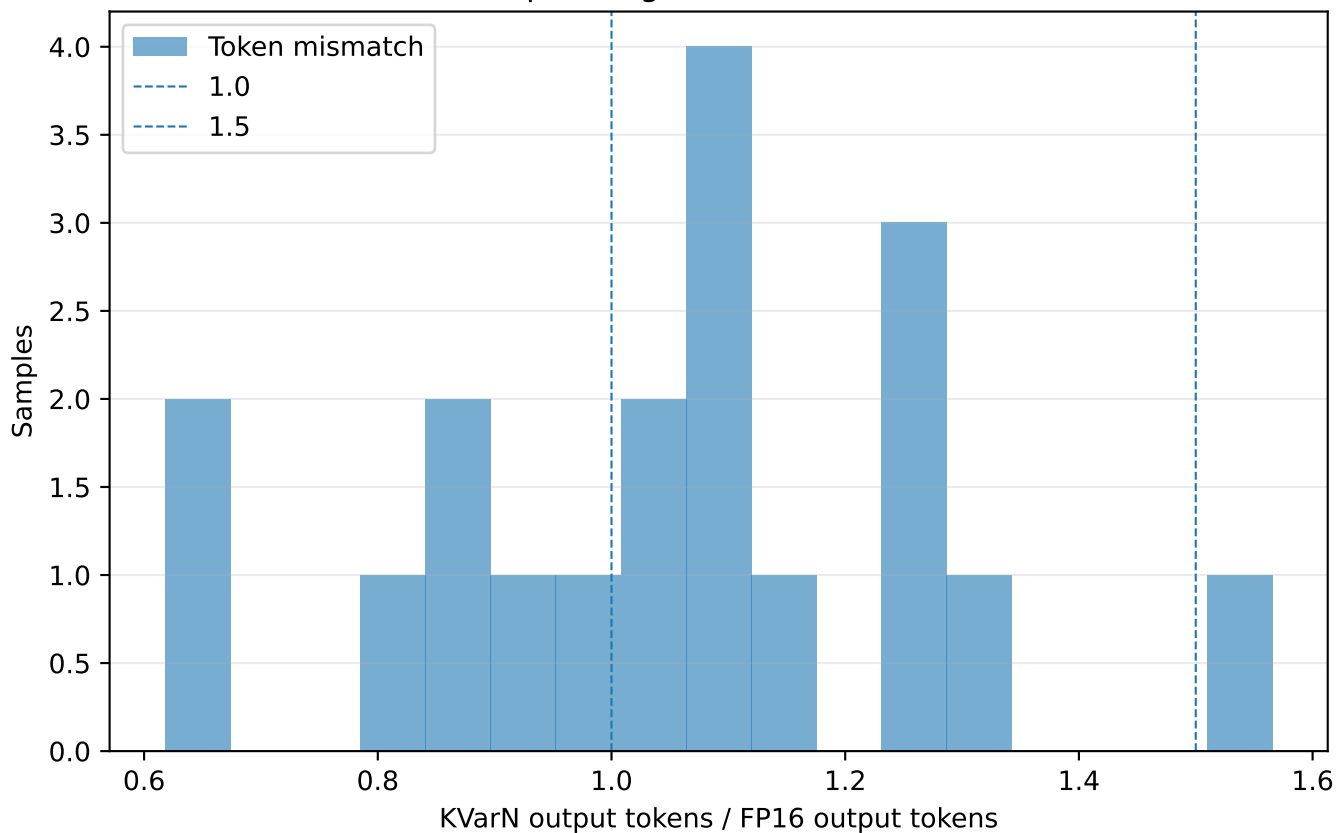
Output-length ratio distribution
