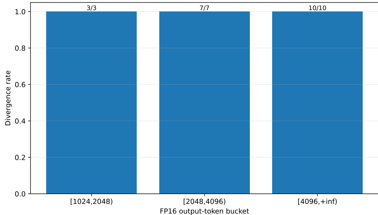
Trajectory divergence versus FP16 output length
