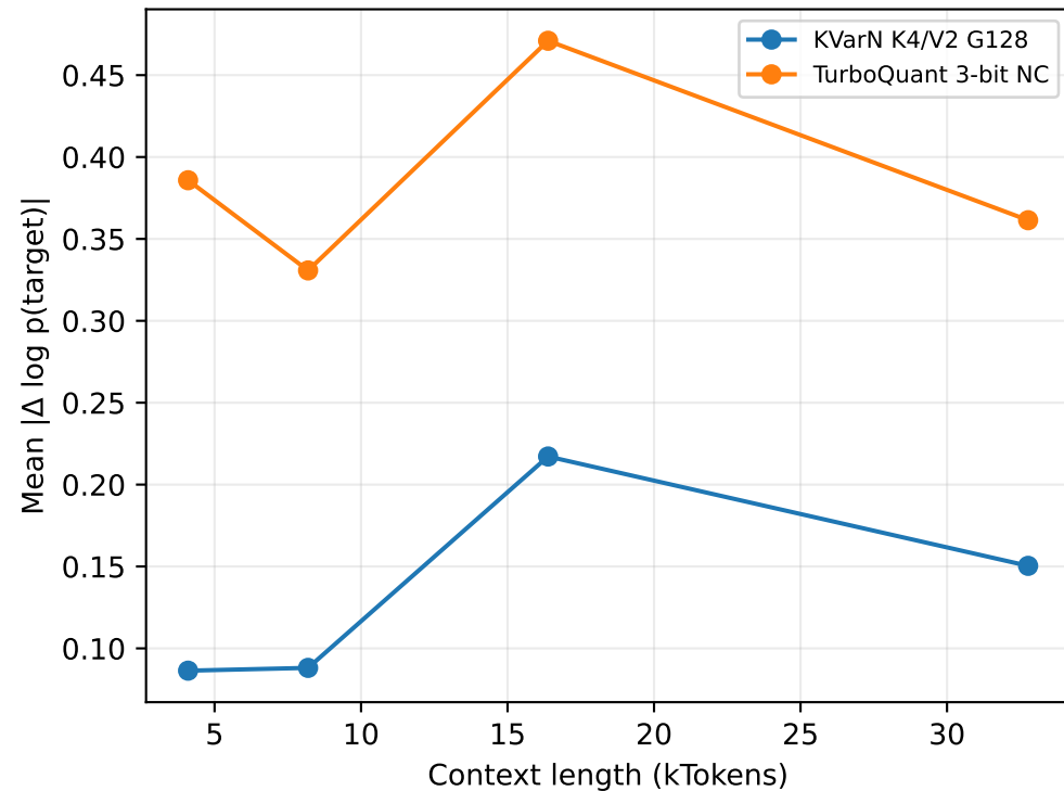
(a) Fixed-trajectory log-probability drift
