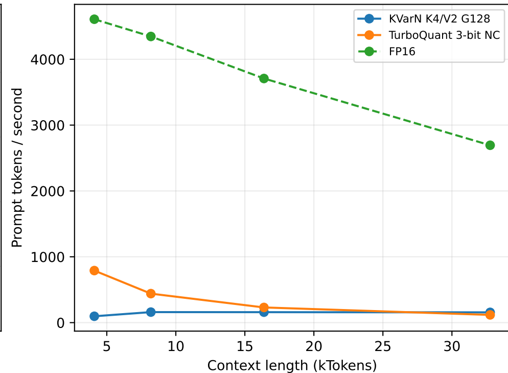
(c) End-to-end prompt scoring throughput
