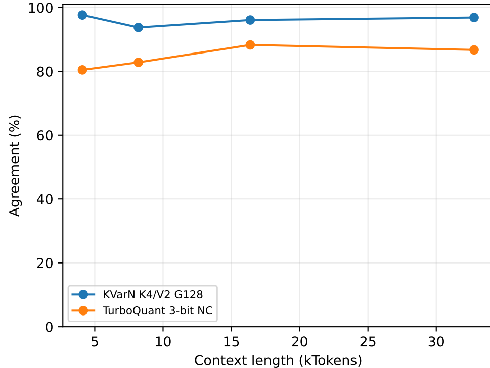
(b) Top-1 agreement with FP16
