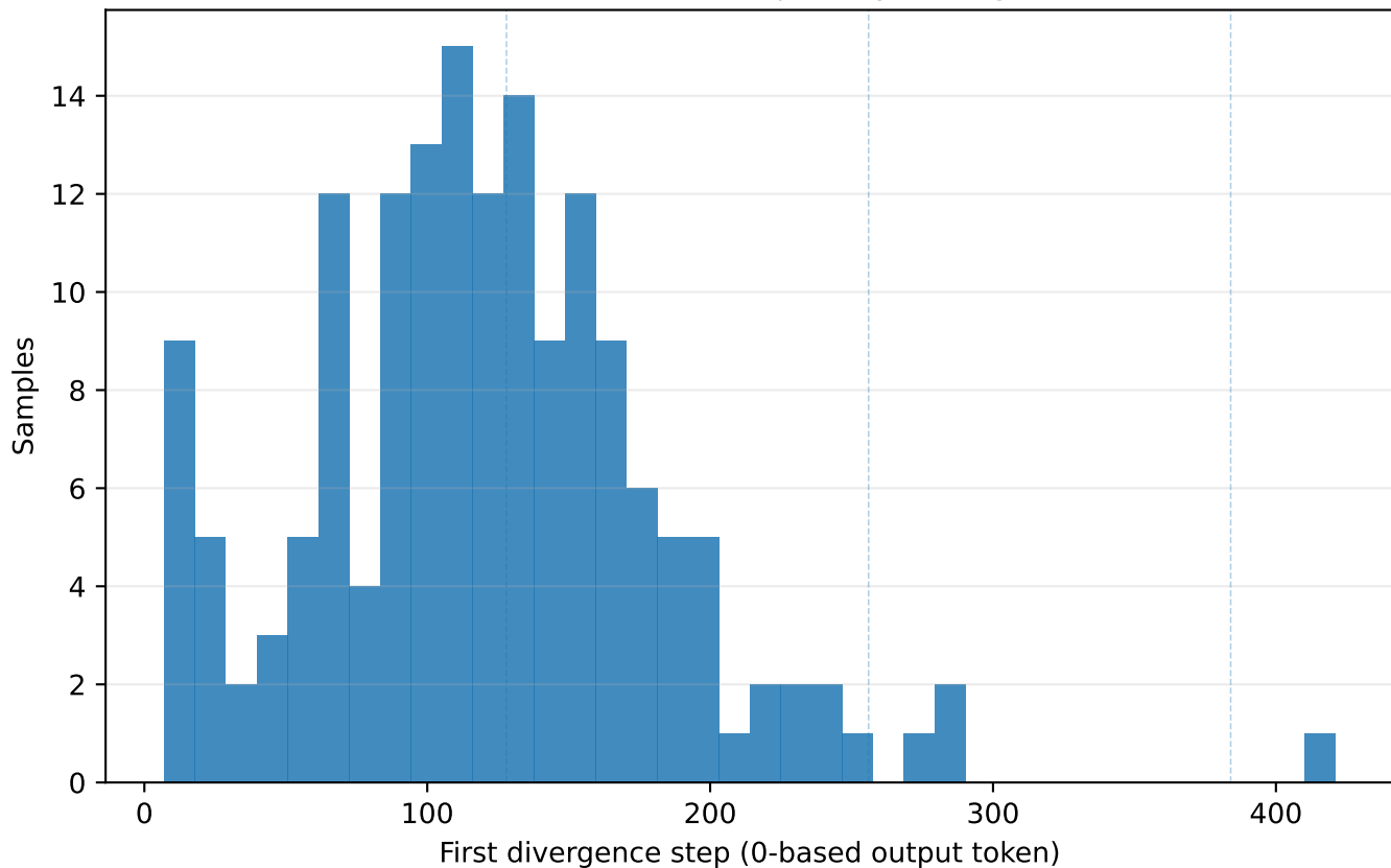
Distribution of first trajectory divergence
