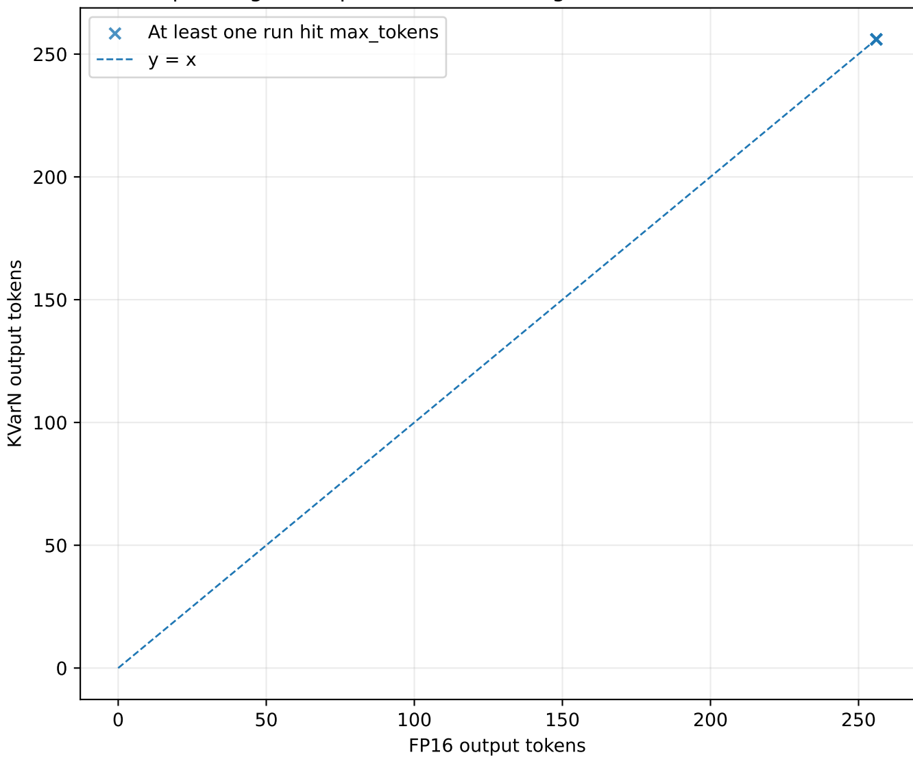
Output length comparison (n=3, divergence=33.3%, censored=3)
