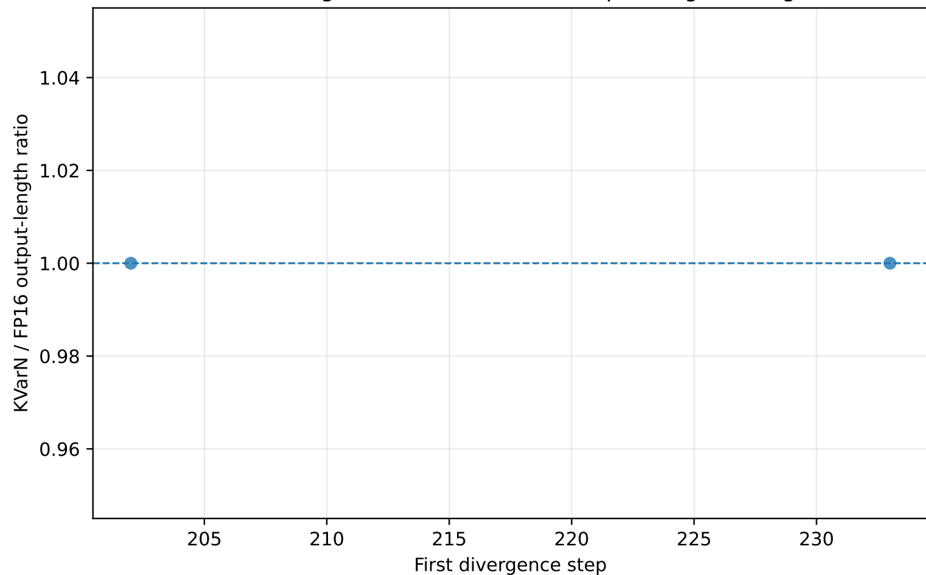
First divergence location versus output-length change
