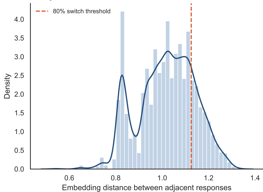
C. Adjacent semantic distance
