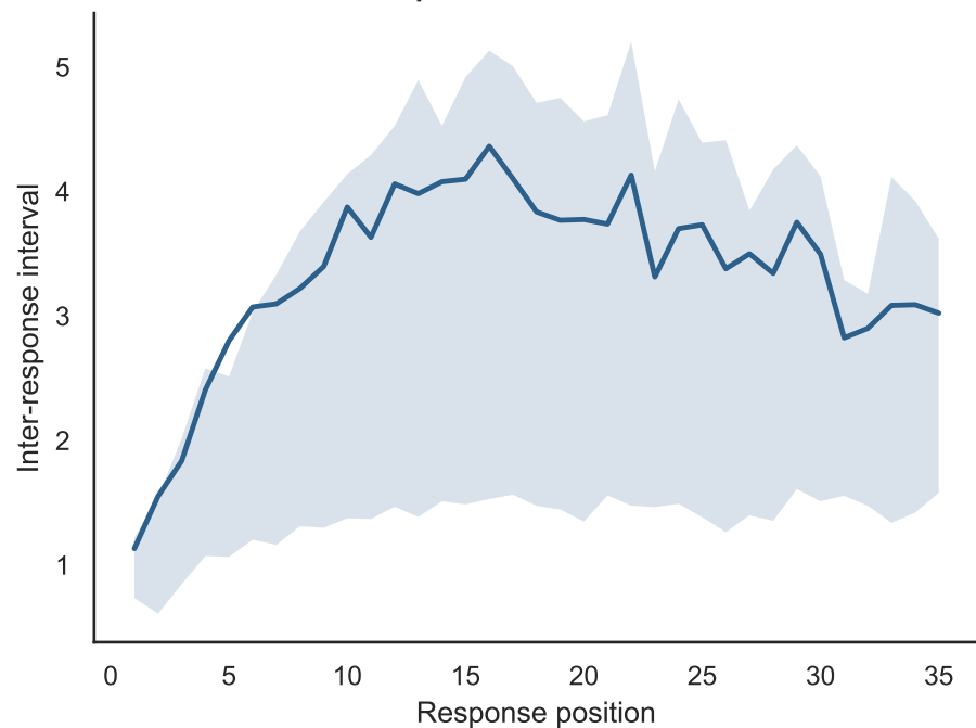
F. Retrieval slows over position
