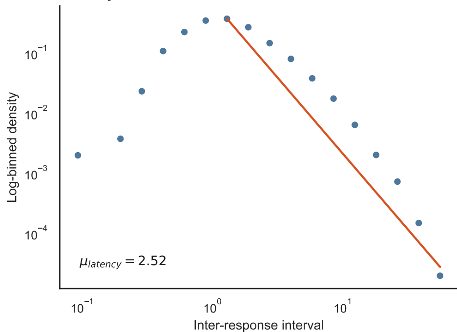
E. Heavy-tailed retrieval latencies
