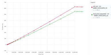
Figure 9: 50% duplicates
