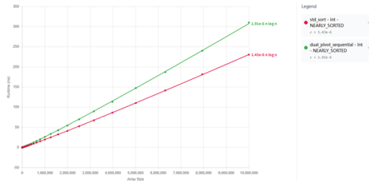
Figure 4: Nearly-sorted
