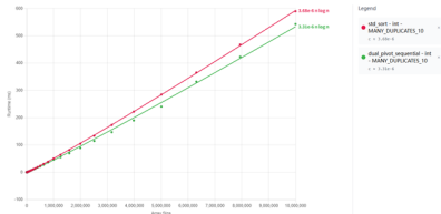
Figure 8: 10% duplicates
