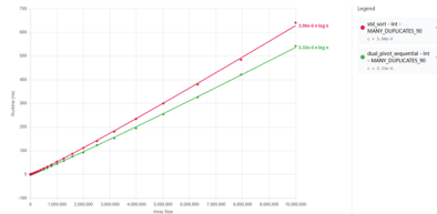
Figure 10: 90% duplicates
