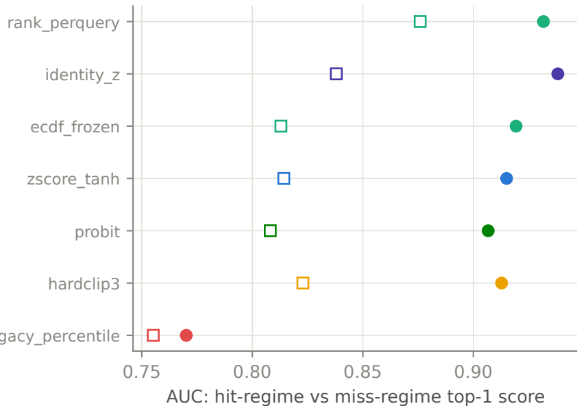
Abstention separability (● libero_10, □ libero_spatial)
