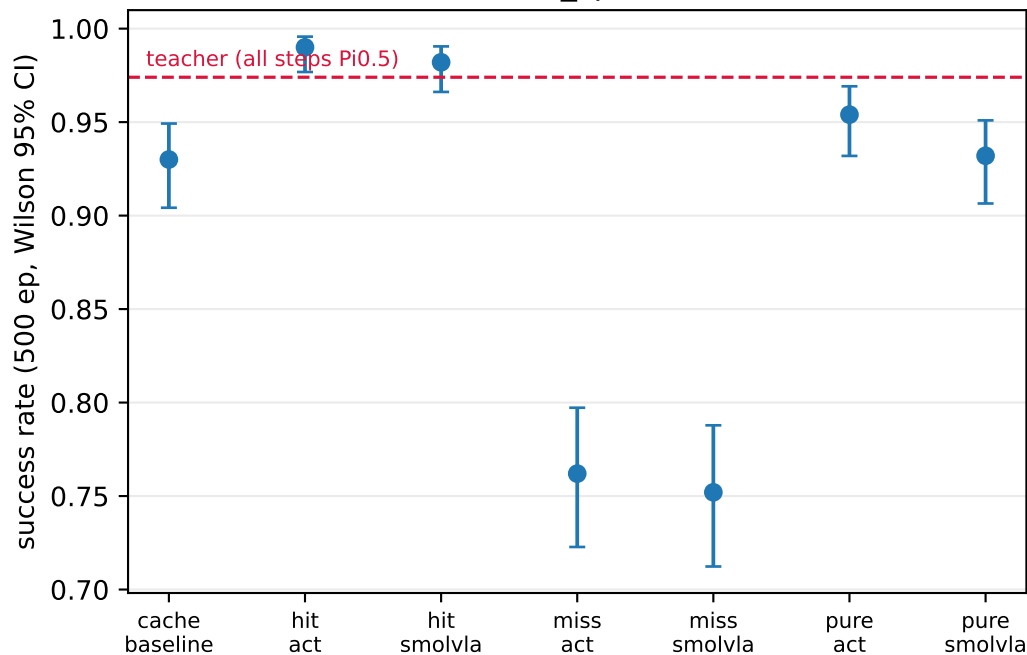
libero_spatial
